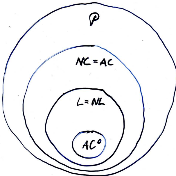
Classes in P
