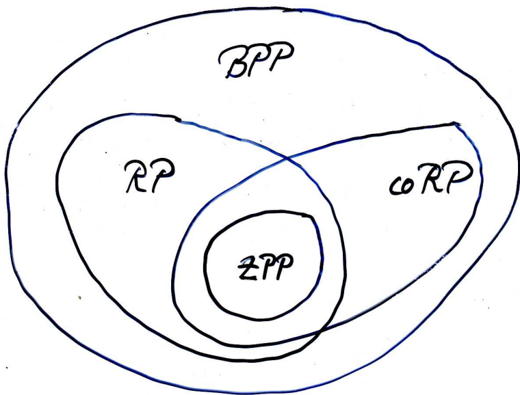
Classes with randomization
